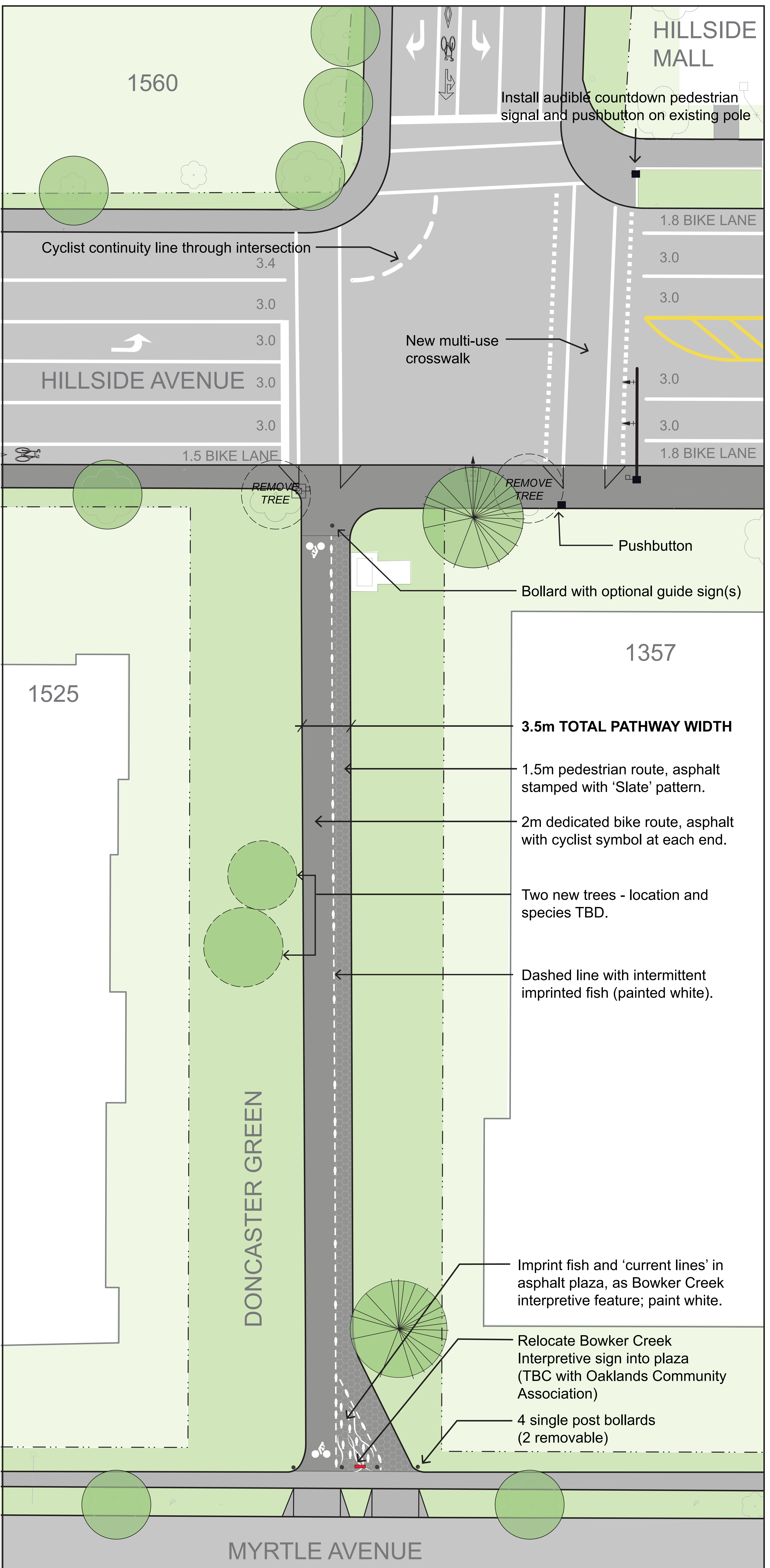
DONCASTER GREENWAY CONNECTION Proposed pathway and intersection improvements
